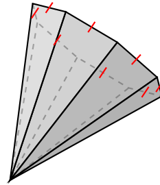
octagonal pyramid
