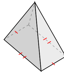
rectangular pyramid
